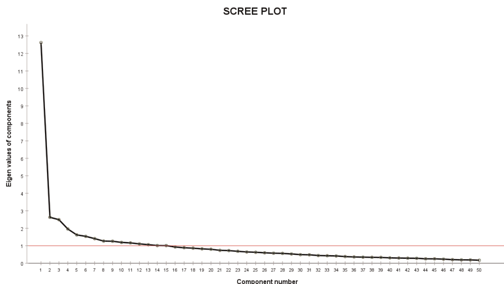
Fig. 1. Eigenvalues of DREEM — scree plot.
