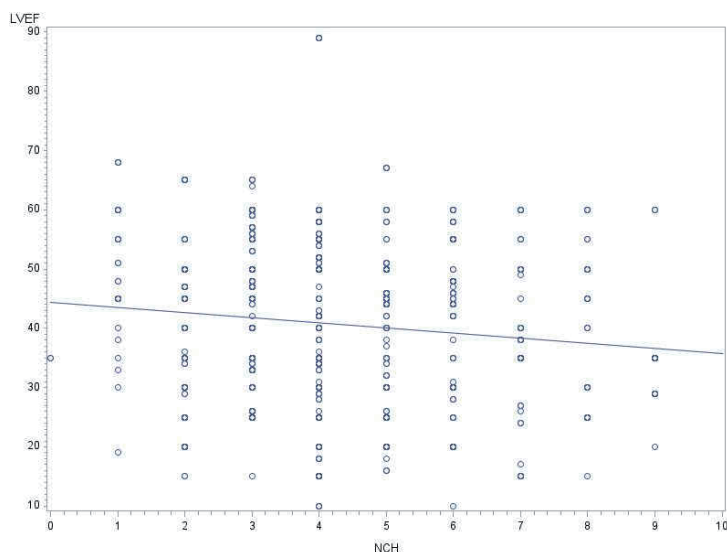
Fig. 2. Association between left ventricular ejection fraction (LVEF) and the total number of co-morbidities (NCH).
